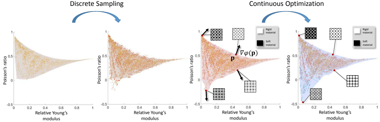
Fig. 4. One cycle of computing the microstructure gamut. Given a set of samples, we compute a signed distance function approximating the material gamut (left) and randomly perturb microstructures lying near the boundary to provide new seeds to the continuous algorithm (middle left). We then update the distance field and use the gradient of the signed distance function at the the boundary to define new target material points (middle right). These target material points are used in a continuous optimization that generates new samples (right).
