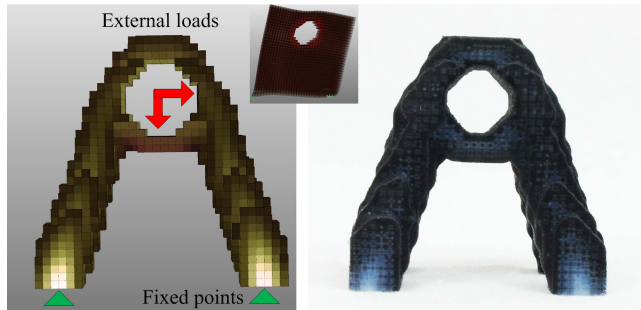
Fig. 20. Optimizing a flexure mount. The flexure is connected to an object thanks to a cylindrical connector. We leave space for this connector by keeping a cylindrical area of the design layout empty of material. The material distribution of the flexure is optimized for two sets of external forces applied to the cylindrical area. Under vertical load, the flexure should stay close to the rest shape while under horizontal load, the flexure should deform according to the inset figure.
