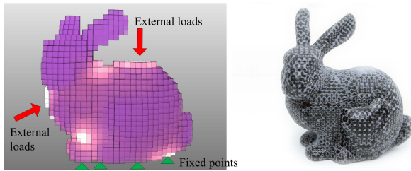
Fig. 22. Stanford bunny optimized for two loading cases. Two sets of external forces are applied to the back and chest of the bunny as indicated by the arrows, and the color indicates the material distribution (left). Material parameters are mapped to microstructures to obtain an object that can be actually printed (right).
