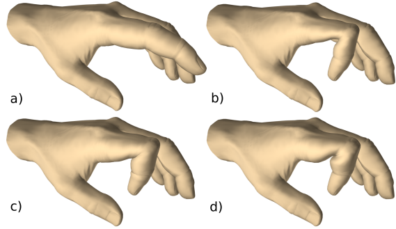
Figure 10: Illustration of the fold-over free application. a) Original mesh. b) Bended finger with classical skinning. c) Simple volume restauration (self-intersection at the junction) d) Fold-over free effect, self-intersections are prevented and the bulge effect is increased.
